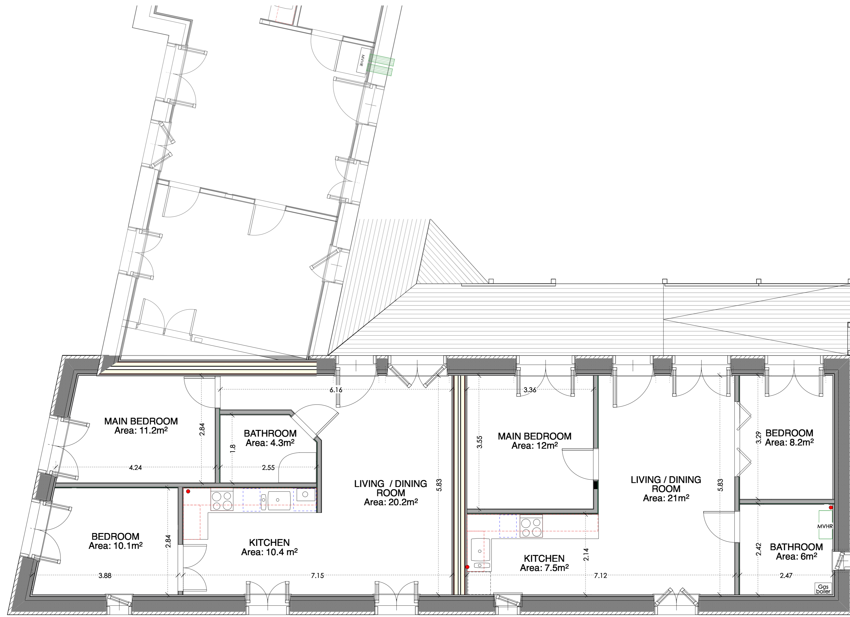
1 FLATS 1-2 FLOOR PLAN S=1:50
