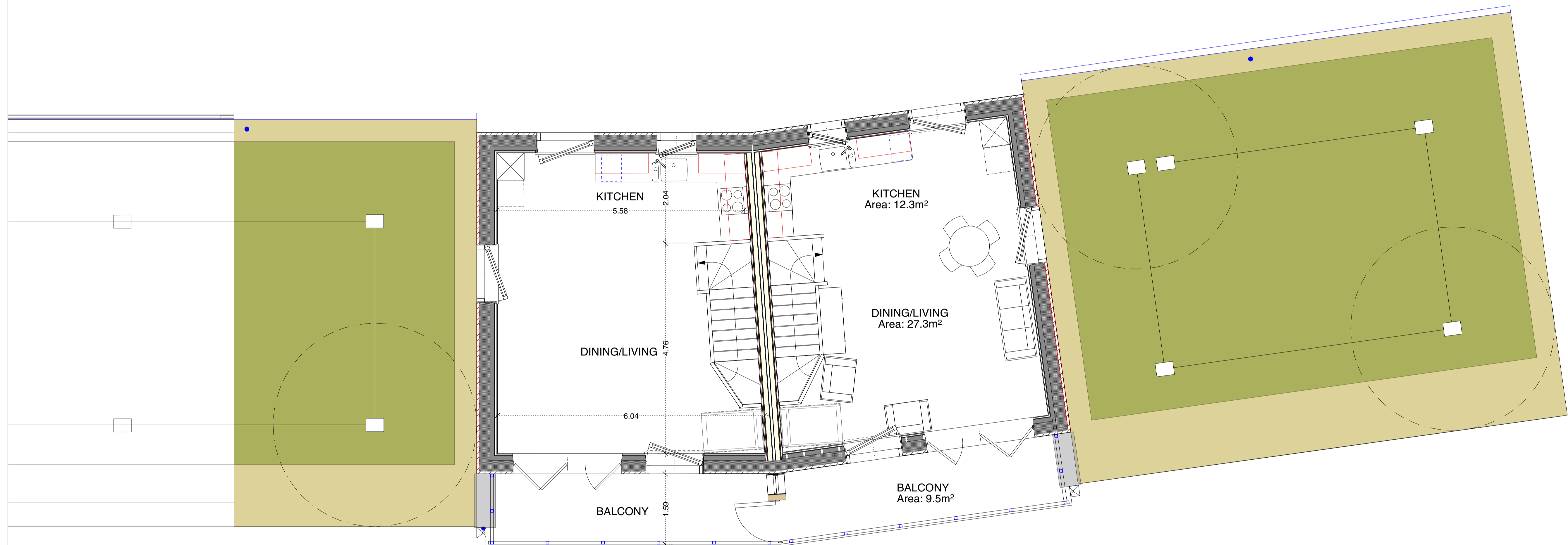
○ HOUSES 7-11 SECOND FLOOR PLANS S=1:50
