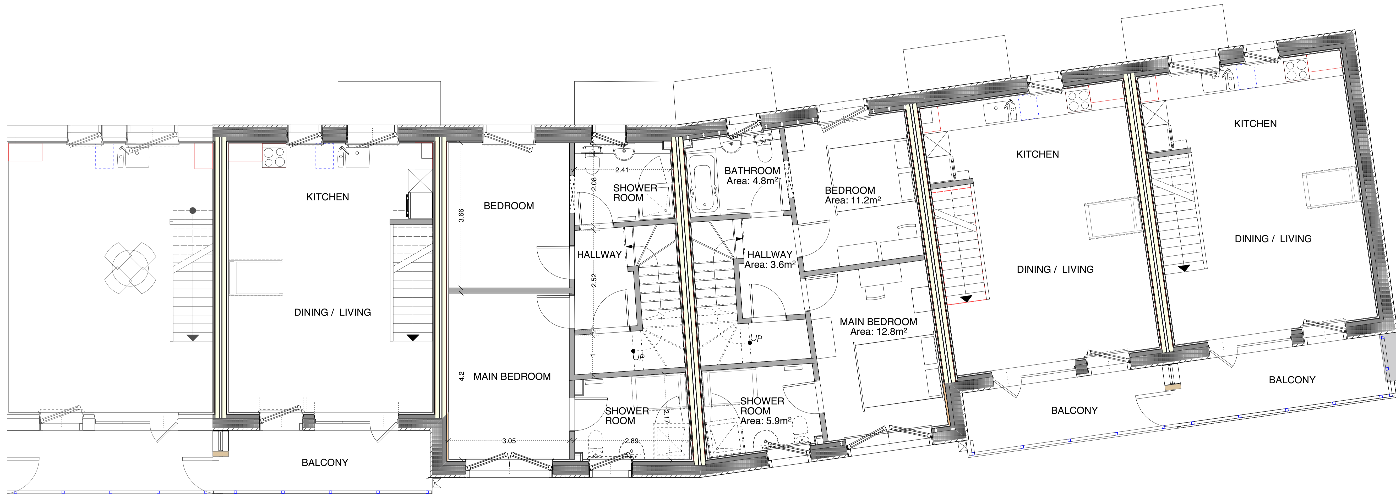
HOUSES 7-11 FIRST FLOOR PLANS S=1:50
