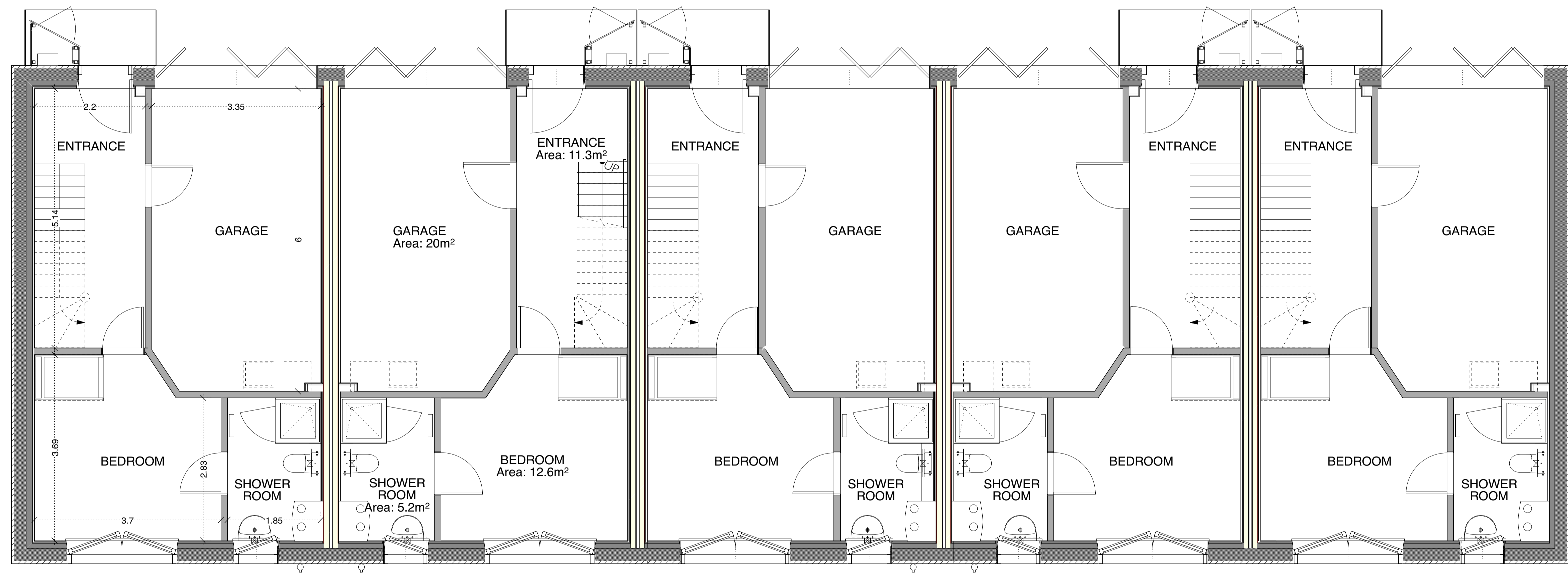
HOUSES 19-23 GROUND FLOOR PLANS S=1:50
