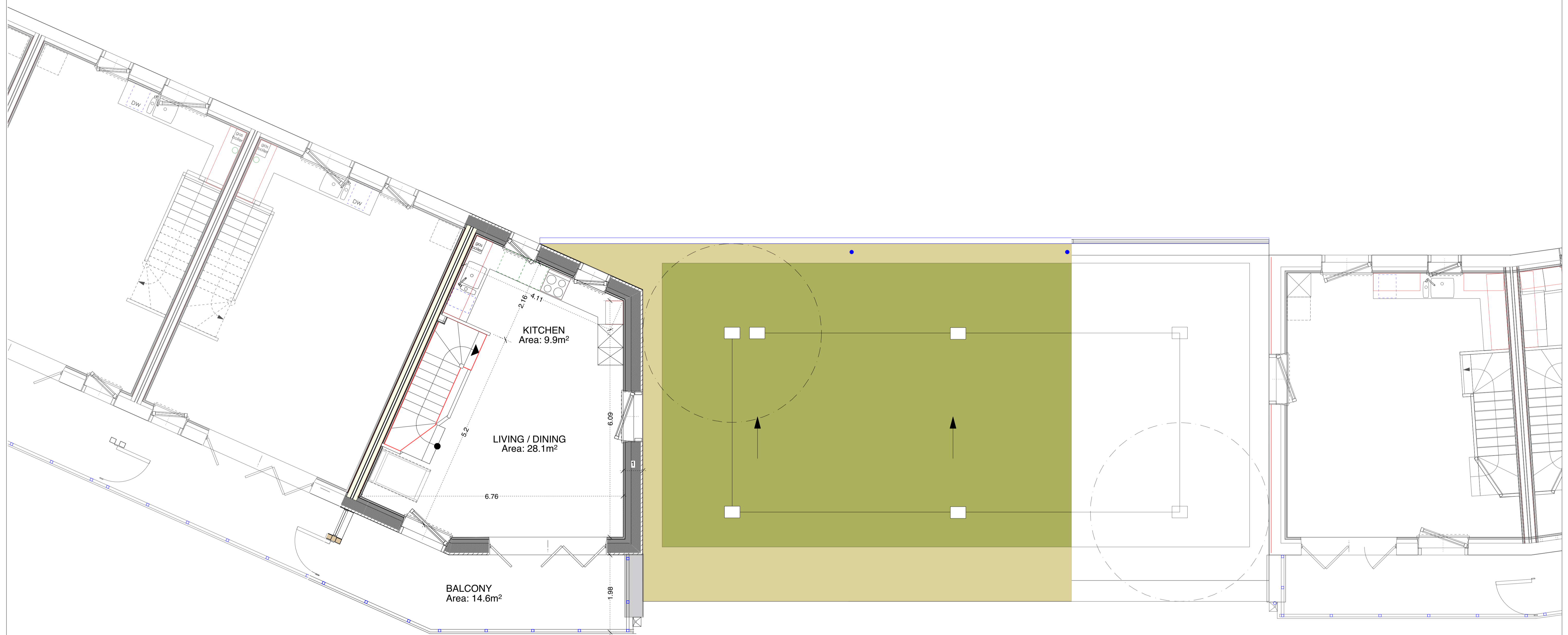
○ HOUSES 12-14 SECOND FLOOR & ROOF PLANS S=1:50
