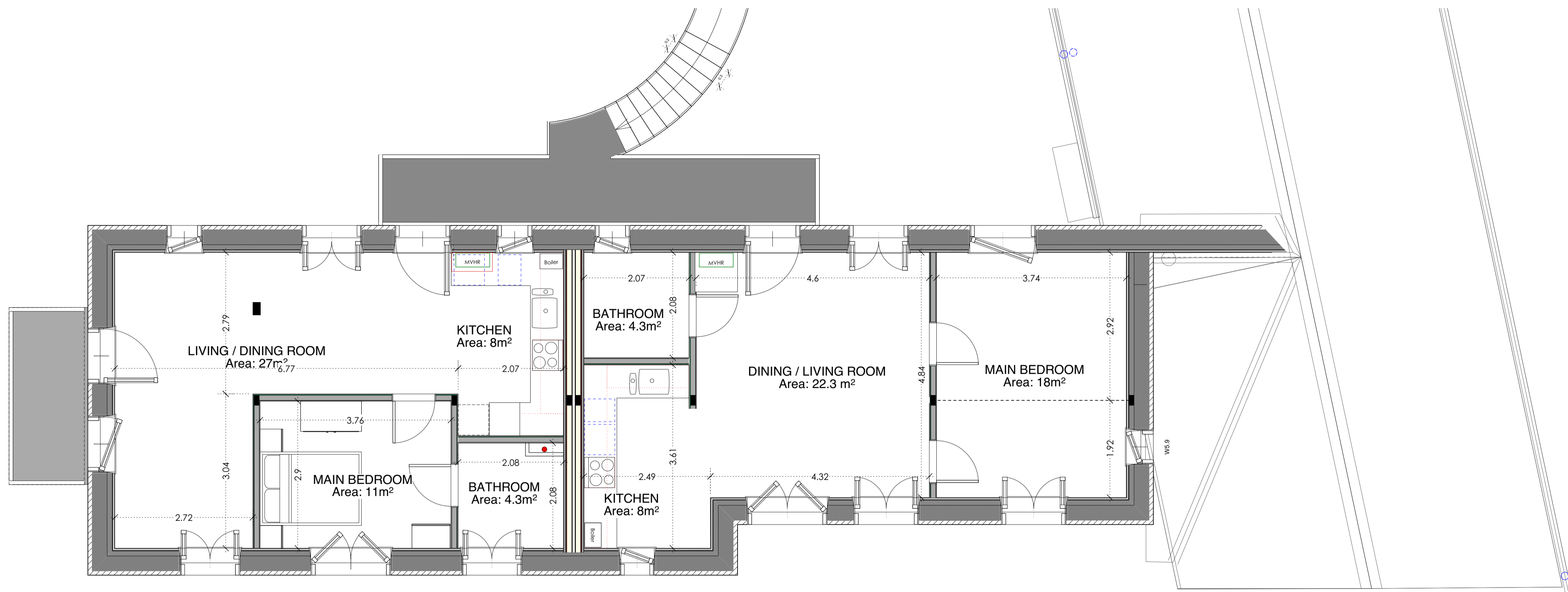
1 5-6 FIRST FLOOR PLAN REAR WING S=1:50
