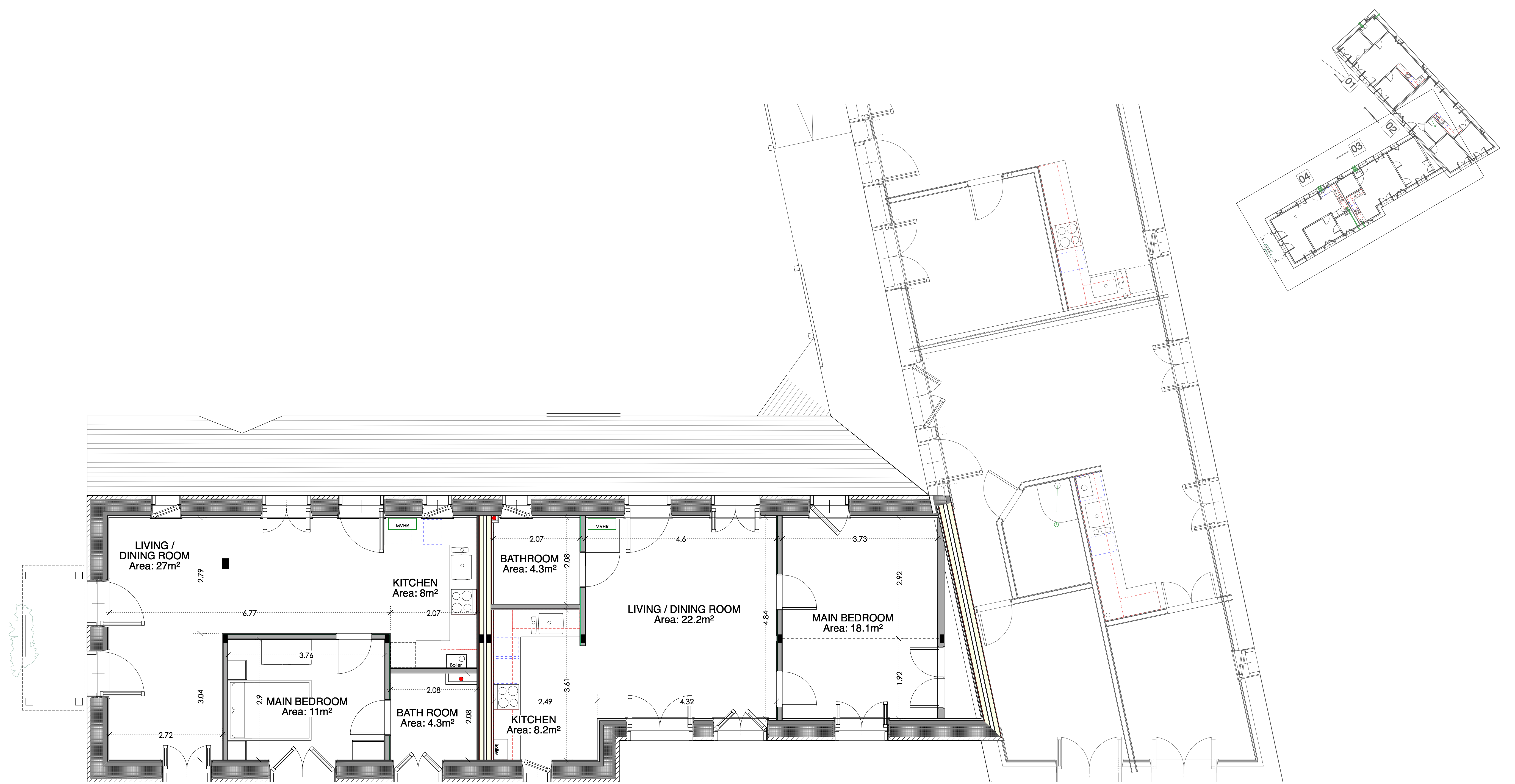
2 FLATS 3-4 FLOOR PLAN S=1:50
